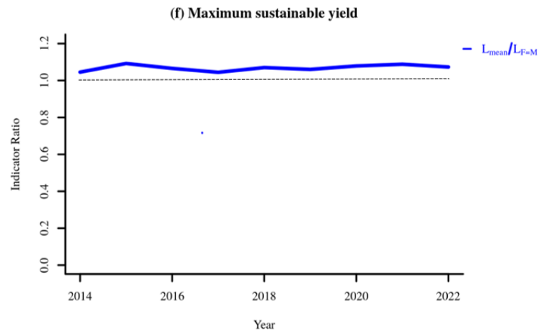
Figure 3.4.10. Flounder in subdivisions 26 and 28 (Eastern Gotland and Gulf of Gdansk). Index ratio L_{mean}/L_{F=M} from the length-based indicator method (LBI; ICES, 2015) used for the evaluation of the exploitation status. The exploitation status is below the F_{MSY} proxy when the index ratio value is higher than 1.
