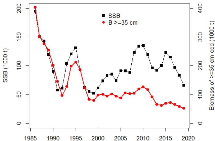
Figure 3 Cod in subdivisions 24–32, eastern Baltic stock. Spawning stock biomass at the spawning time and biomass of commercial sized cod ( \geq 35 cm in length) in the beginning of the year.
